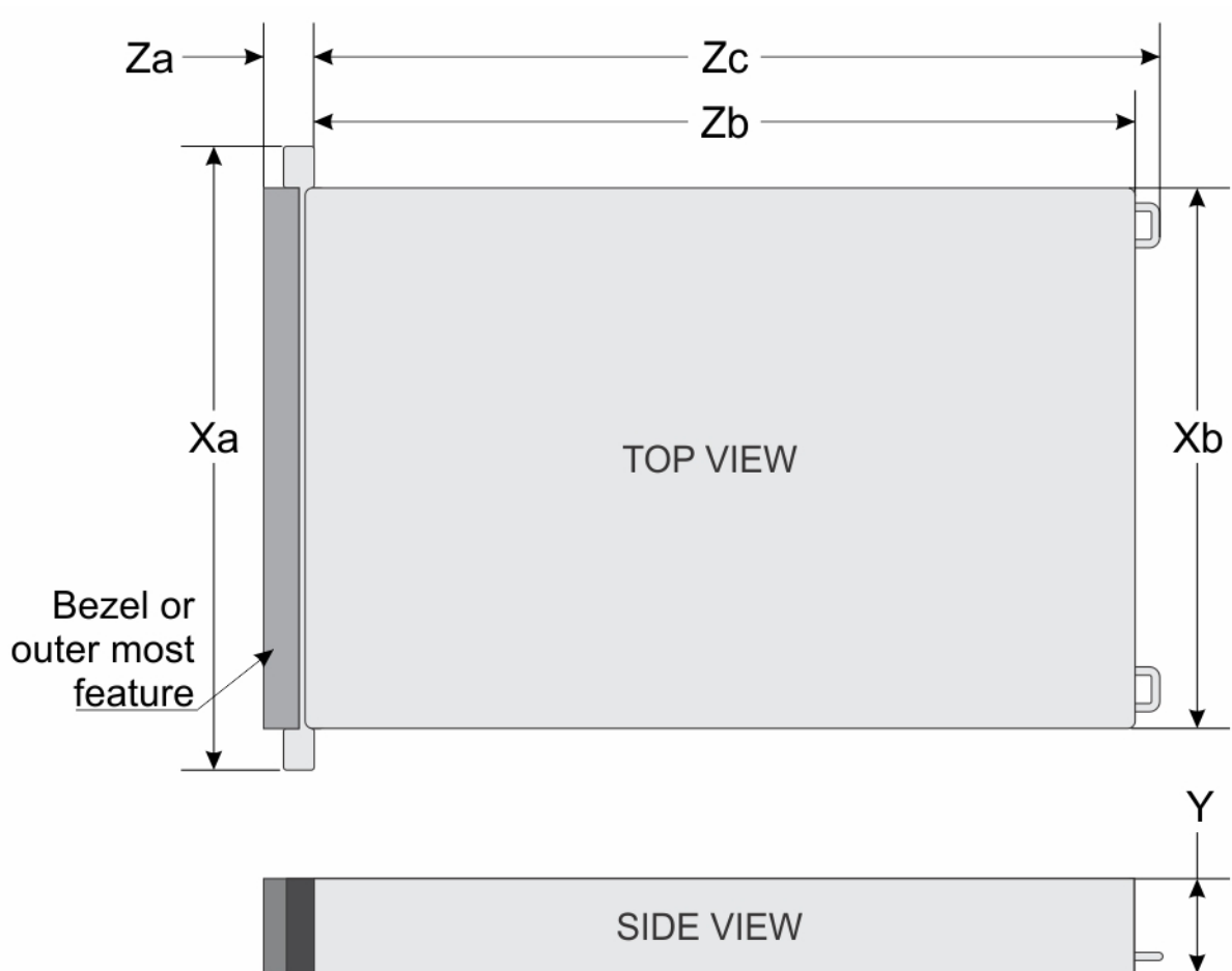
Figure 53. Chassis dimensions
