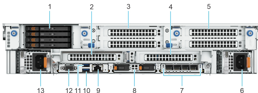
Figure 17. Rear view of the system with rear EDSFF E3.S NVMe drives
