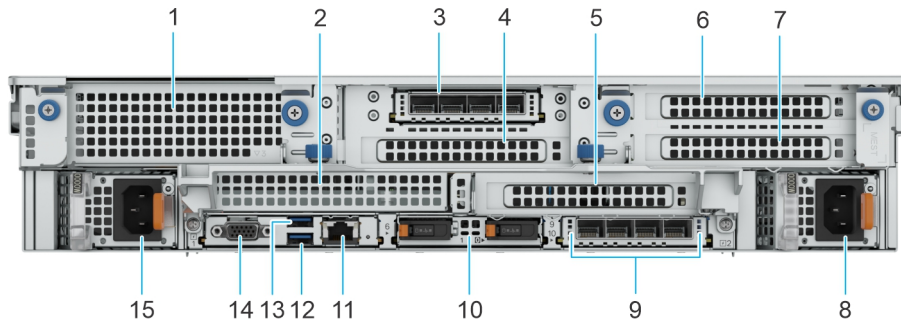
Figure 18. Rear view of the no backplane configuration system
